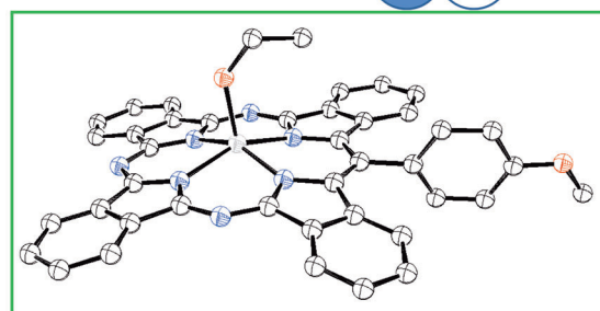
Scheme 5. Efficient synthesis of the magnesium meso-(4-methoxyphenyl) TBTP 5 and its X-ray crystal structure. Thermal ellipsoids shown at 50% probability.
